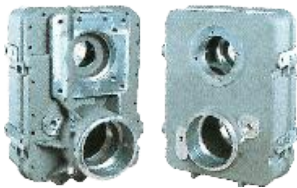
HOUSING FOR GEARBOX G64C
